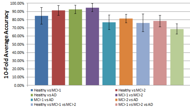
Fig. 4. Bar chart of the highest performing results for each test case using RFE. Error bars correspond to 95% CI.
