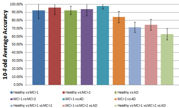
Fig. 3. Bar chart of the highest performing results for each test case using Elastic-net technique for feature selection. Error bars correspond to 95% CI.
